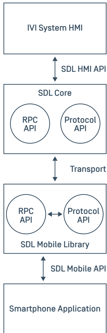
Data Flowchart
